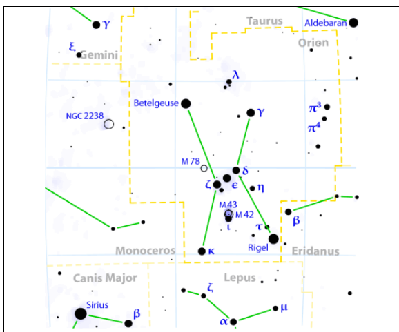
Orión (Orion)
