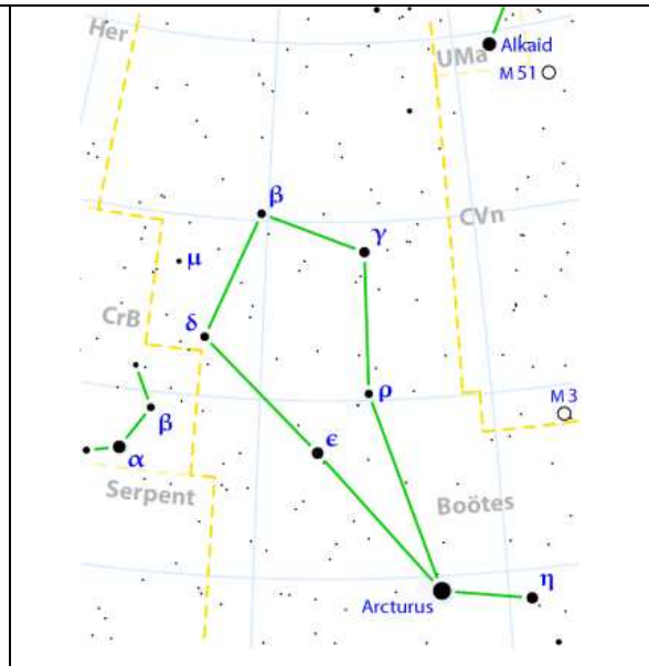
Boyero (Bootes)
