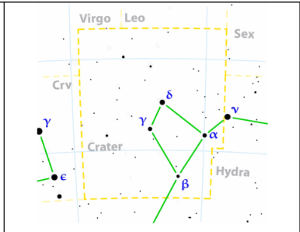
Copa (Crater)
