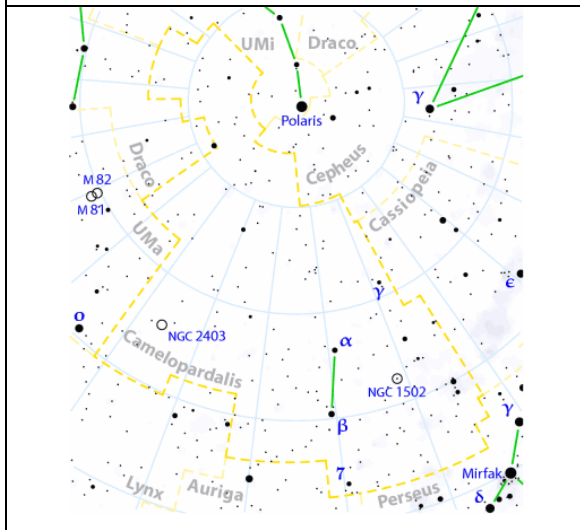
Jirafa (Camelopardalis)
